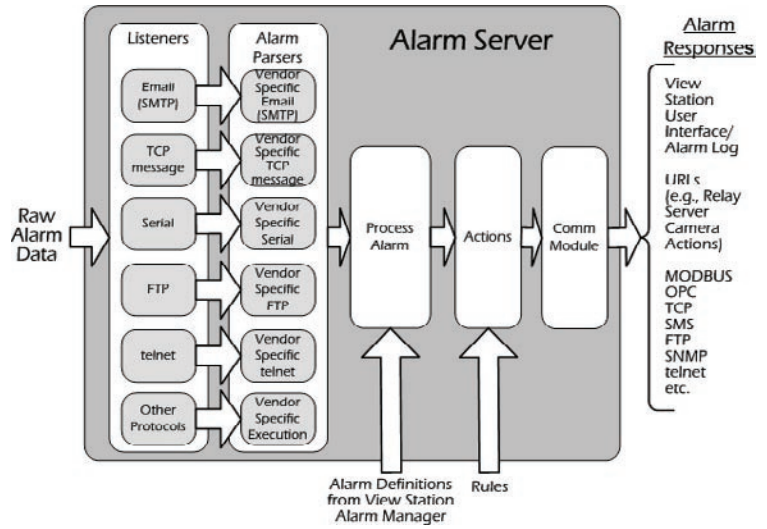
Alarm Server Functional Diagram
